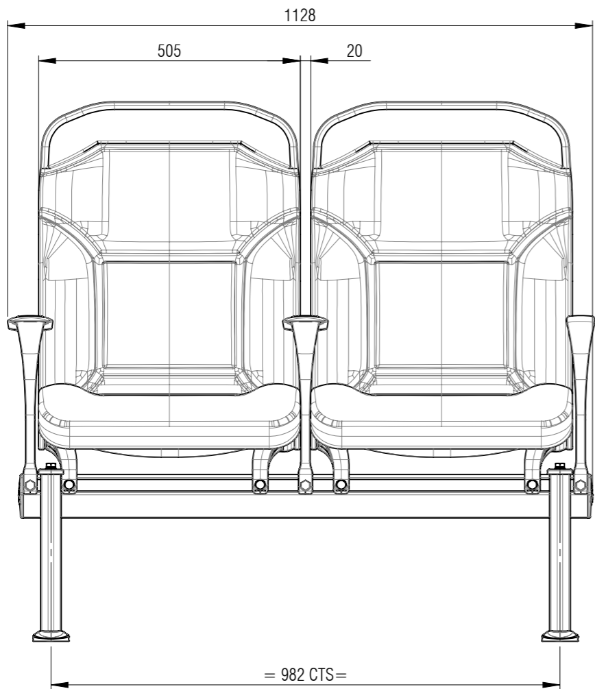
FRONT VIEW
